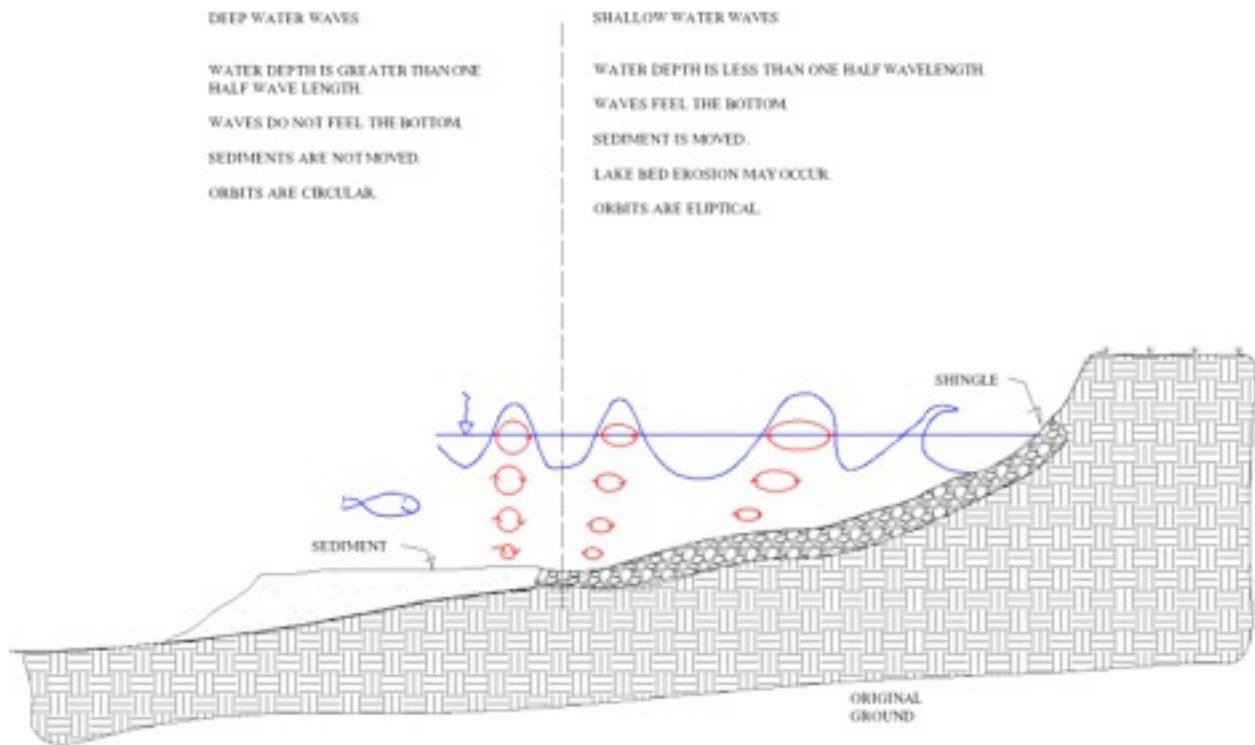
Figure 1 Typical Lake Shoreline Cross Section 3
